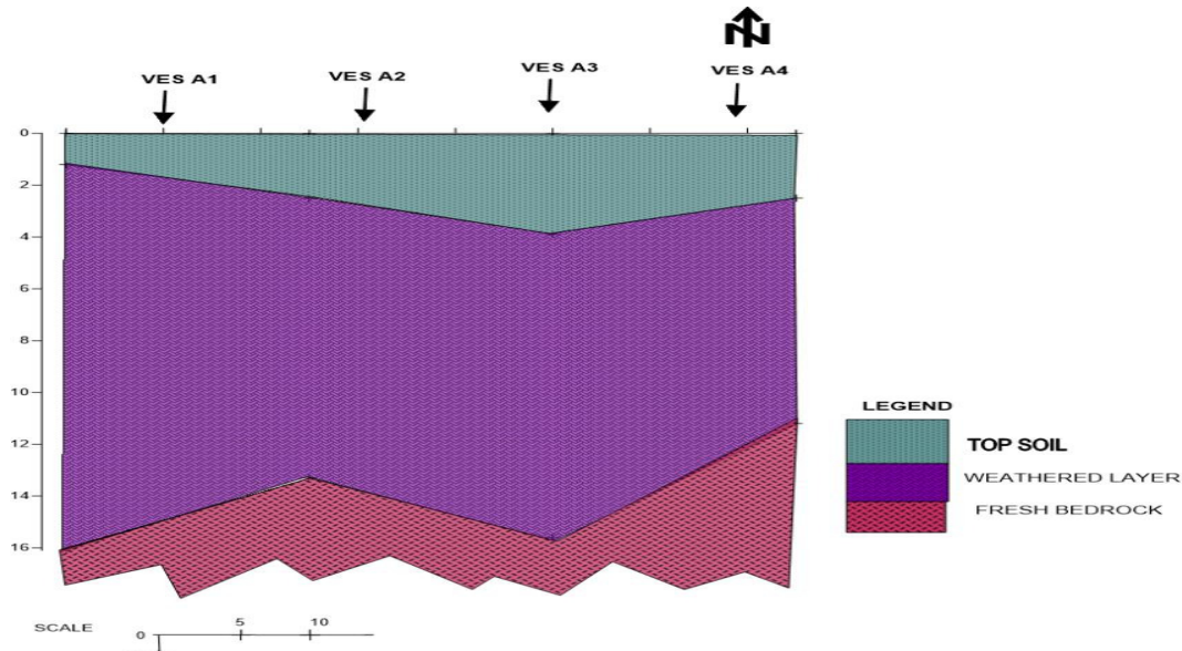
Figure 8: Geo-electric section.
