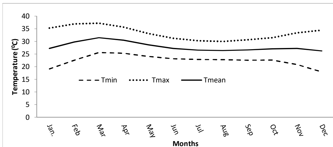
Figure 5: Monthly in Minimum, Maximum and Mean Temperatures over Fiidi, Makurdi (1986-2016)
