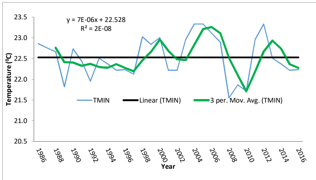
Figure 2: Annual Variation in Minimum Temperature over Fidi, Makurdi (1986-2016)
