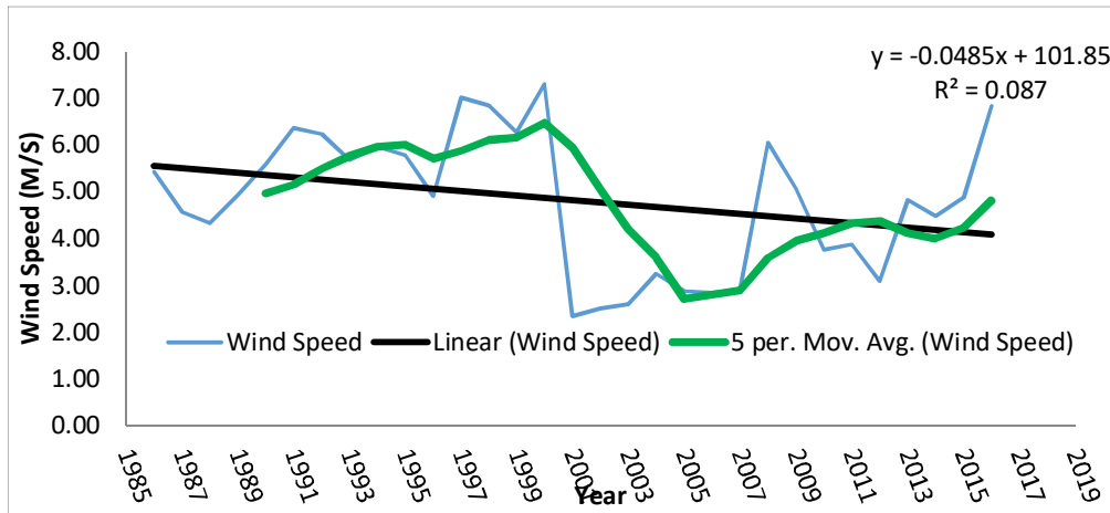
Figure 7: Annual Variation in Wind Speed over Fiidi, Makurdi (1986-2016)
