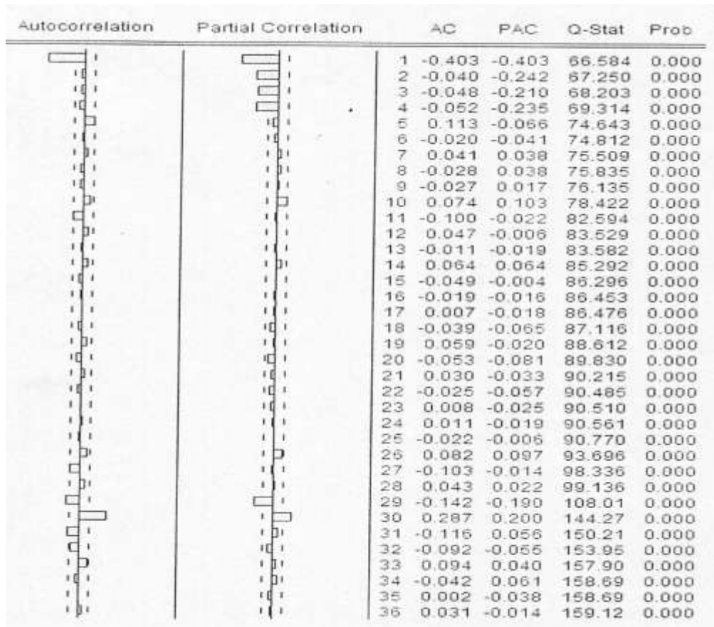
Figure 4: ACF and partial ACF Plots of the Differenced Logged – data
