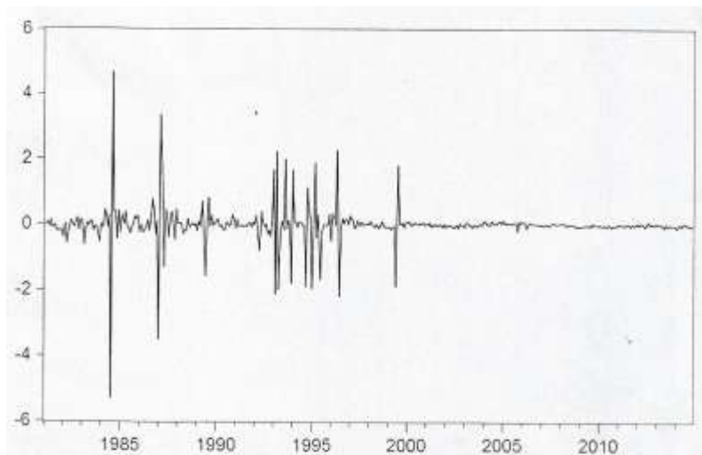
Figure 3: Difference of Log of Nigerian External Reserves
