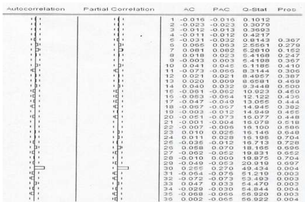
Figure 5: Correlogram of Residuals
