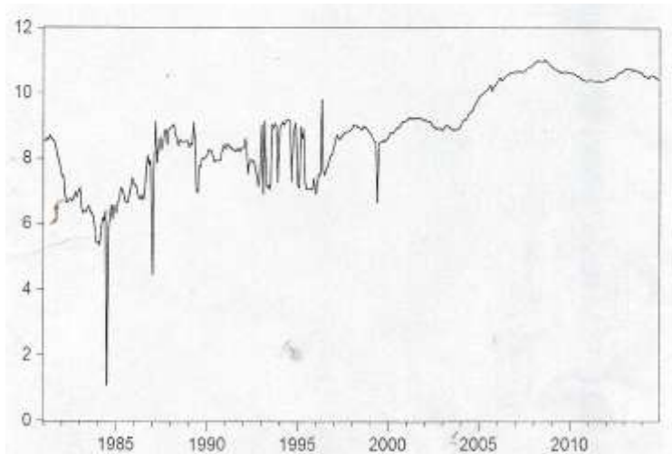
Figure 2: Logarithm of Nigerian External Reserves
