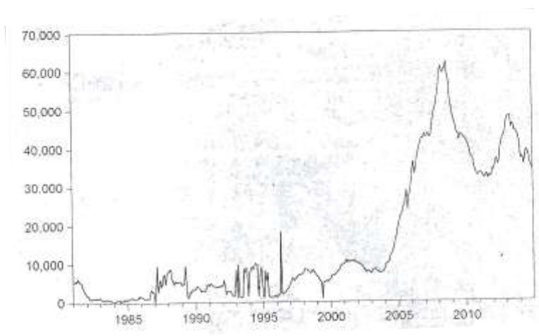
Figures 1: Time Plot of Nigerian External Reserves
