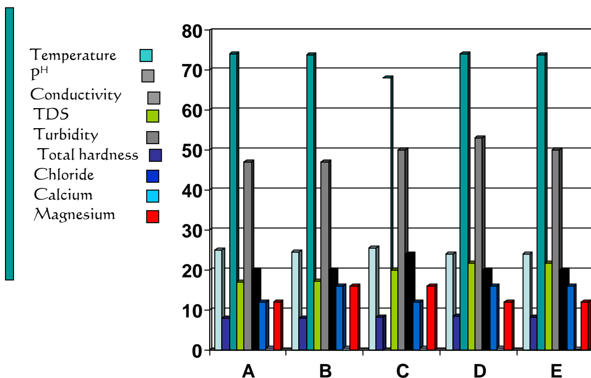
Fig II: Histogram Distribution of Samples
