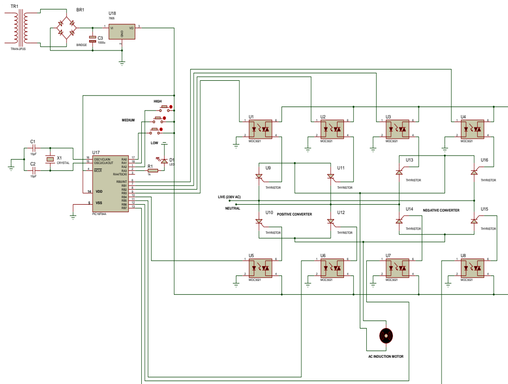
Figure 5. Complete circuit of the cycloconverter.
